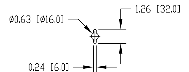
DETAIL "D"
