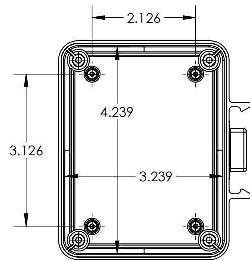
INSIDE VIEW OF BASE
