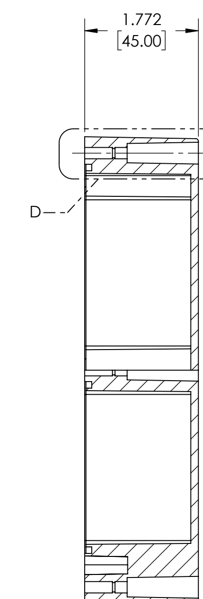
SECTION C-C
