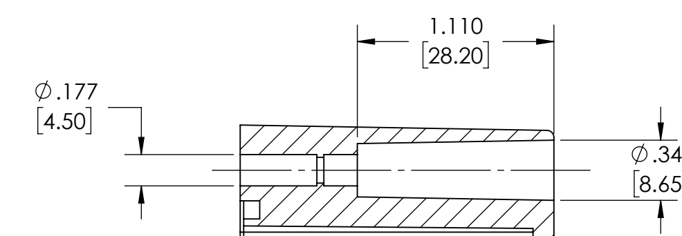
DETAIL D SCALE 2:1.5
