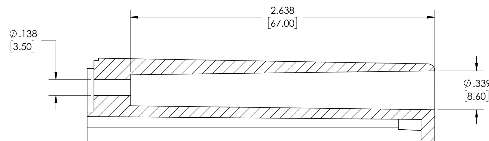
DETAIL B
