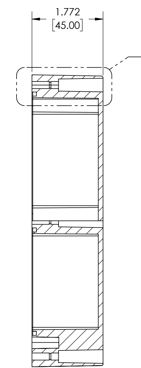
SECTION C-C
