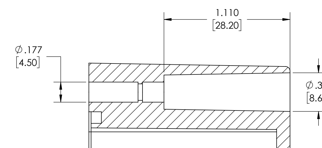
DETAIL D
