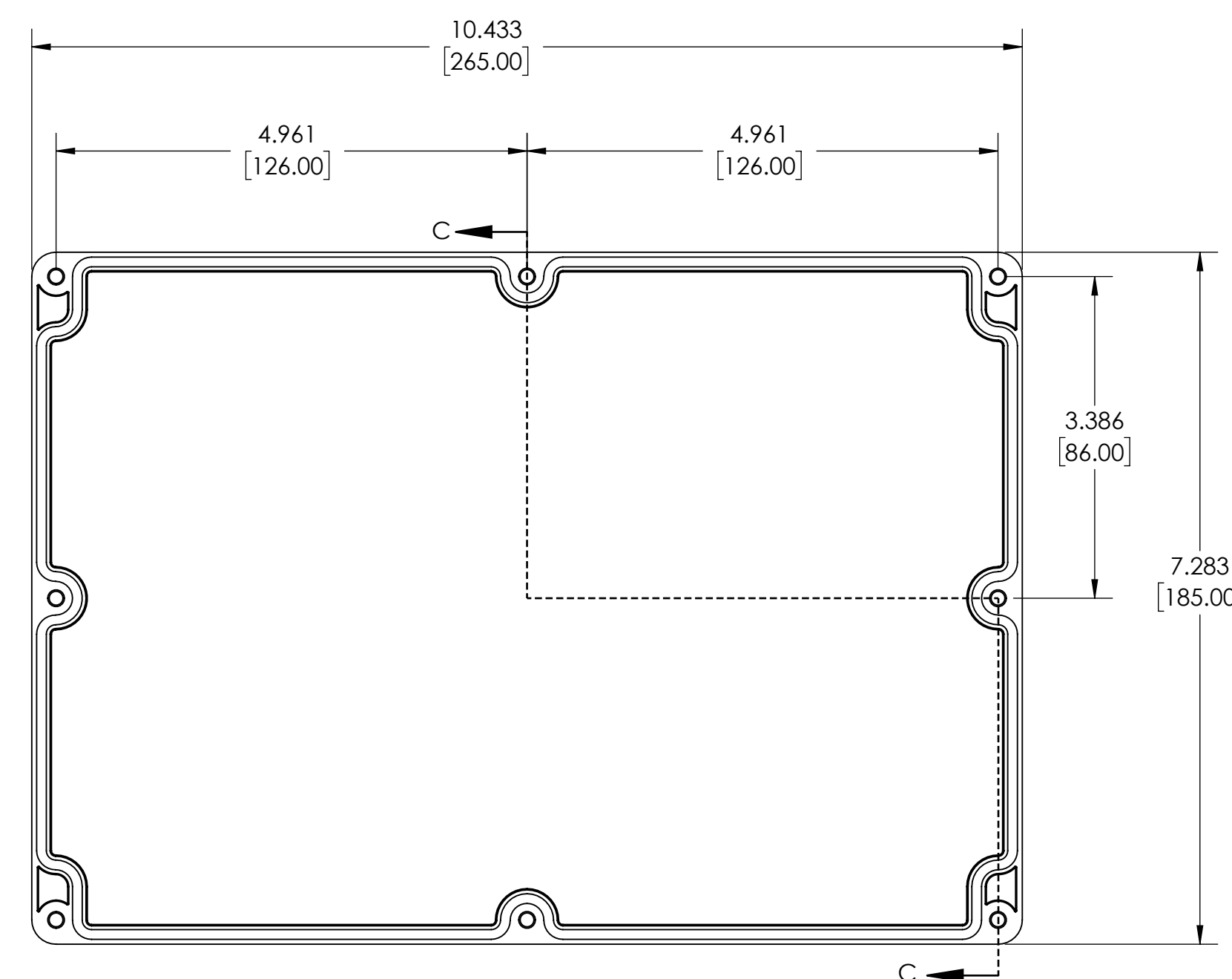
COVER
