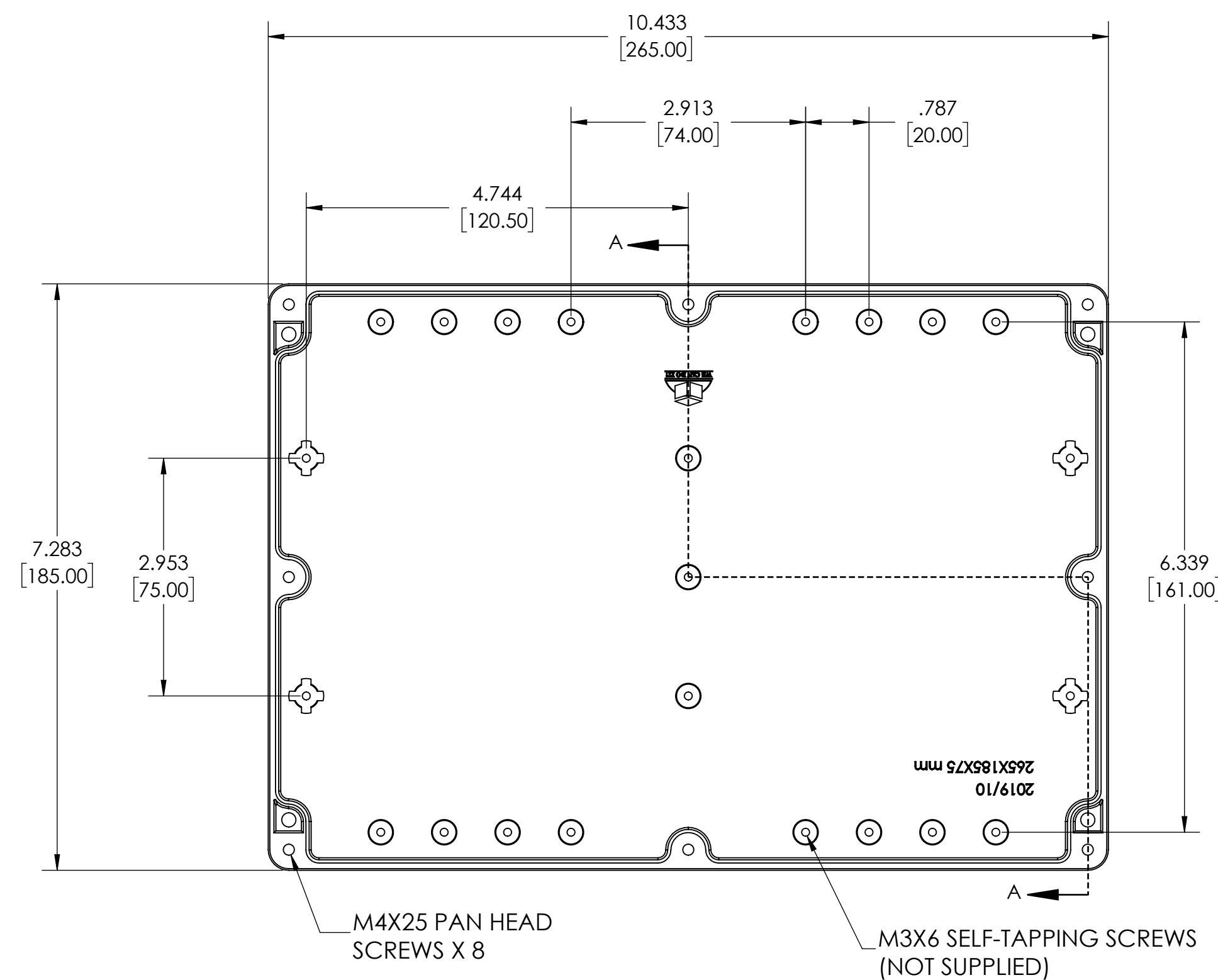
BODY
