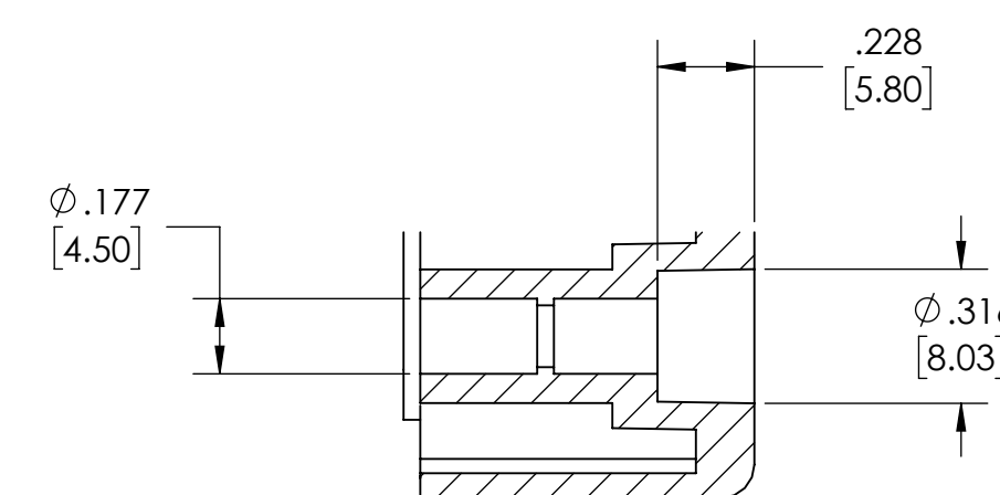
DETAIL D
