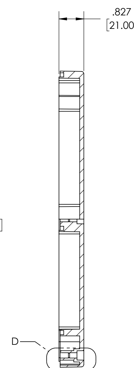
SECTION C-C
