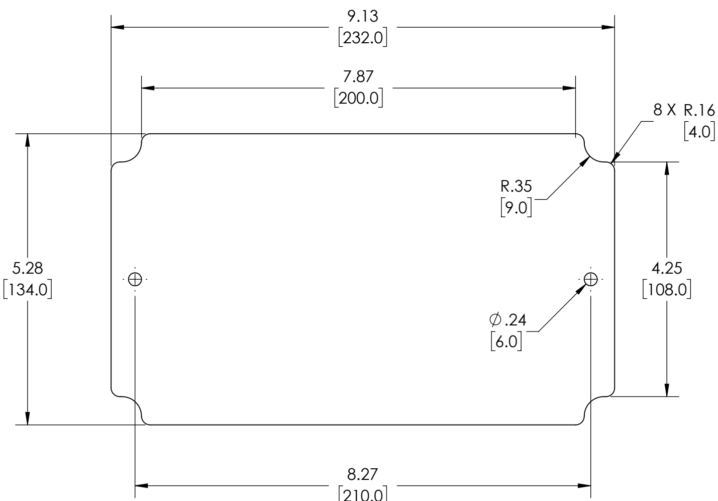
OPTIONAL INTERNAL PANEL AND SUGGESTED PC BOARD LAYOUT
