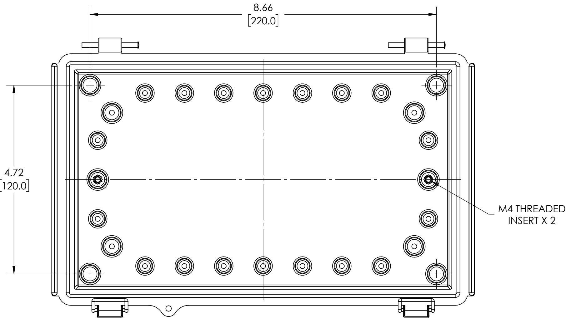
INSIDE VIEW OF BASE
