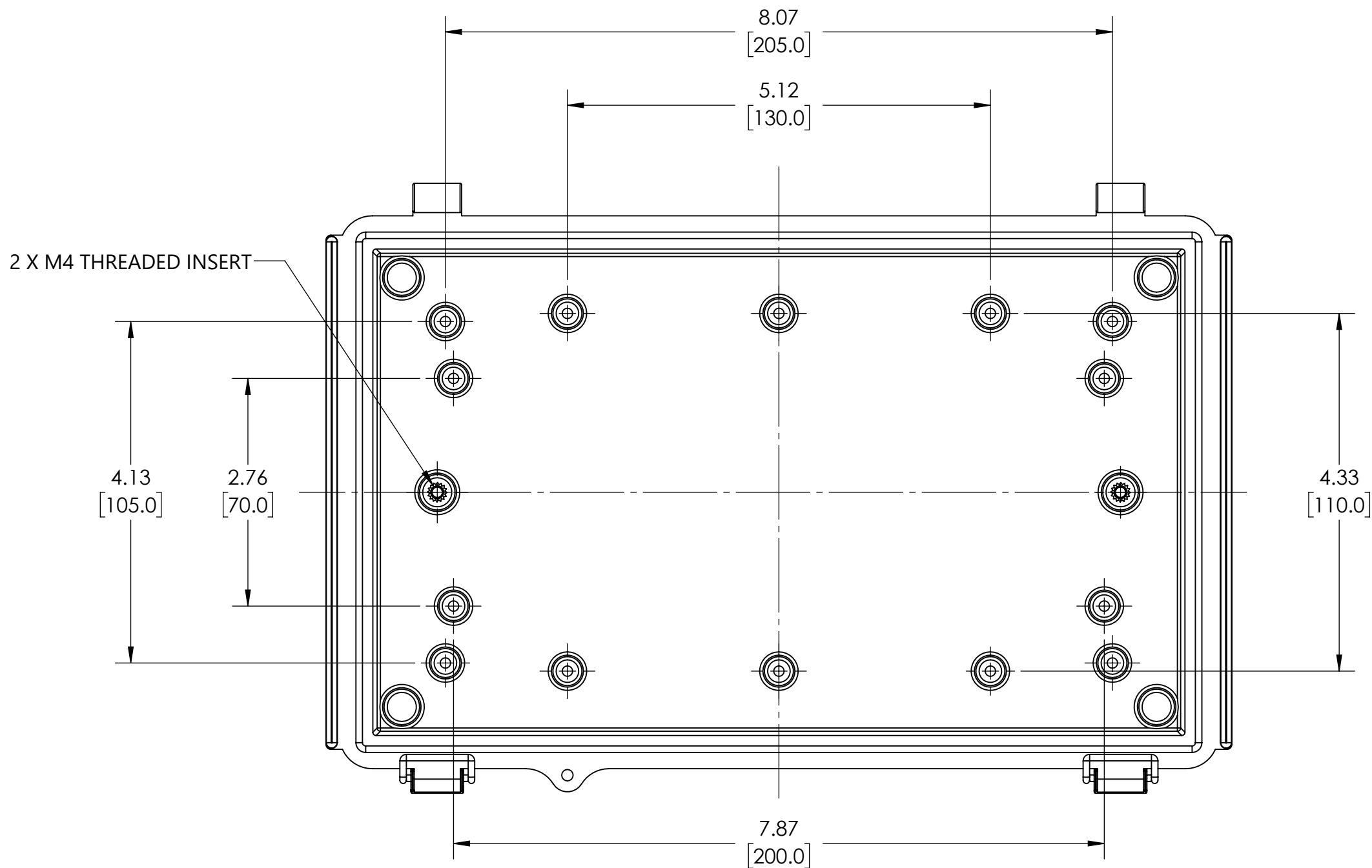
INSIDE VIEW OF BODY
