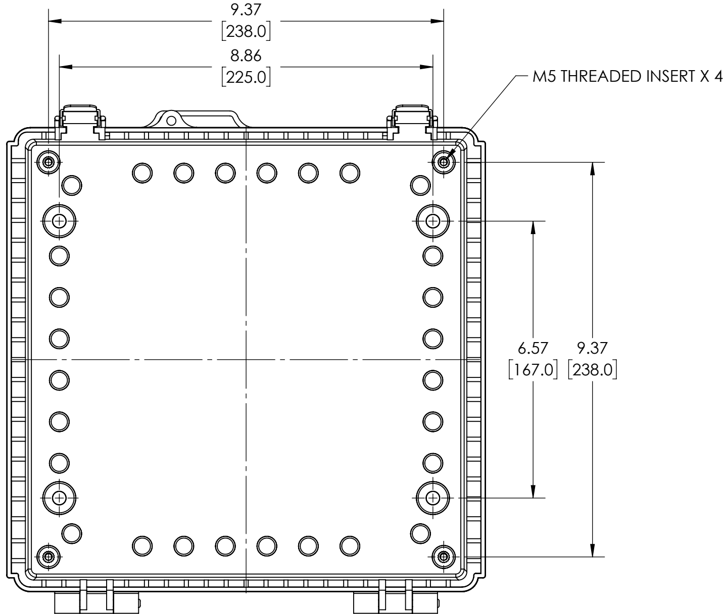
BOTTOM VIEW
