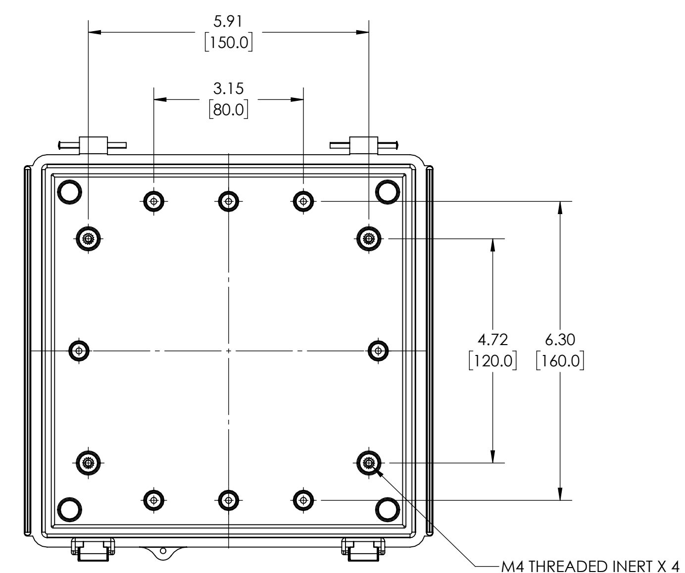
INSIDE VIEW OF BASE
