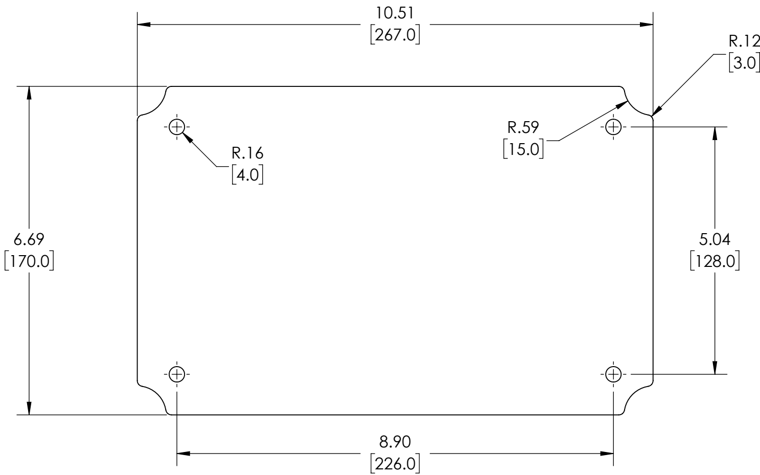
OPTIONAL INTERNAL PANEL AND SUGGESTED PC BOARD LAYOUT
