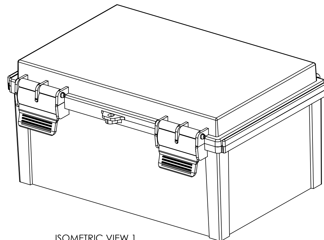
ISOMETRIC VIEW 1
